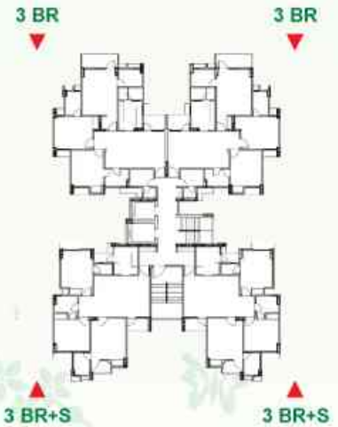
Block-G,H&Q Typical Floor
